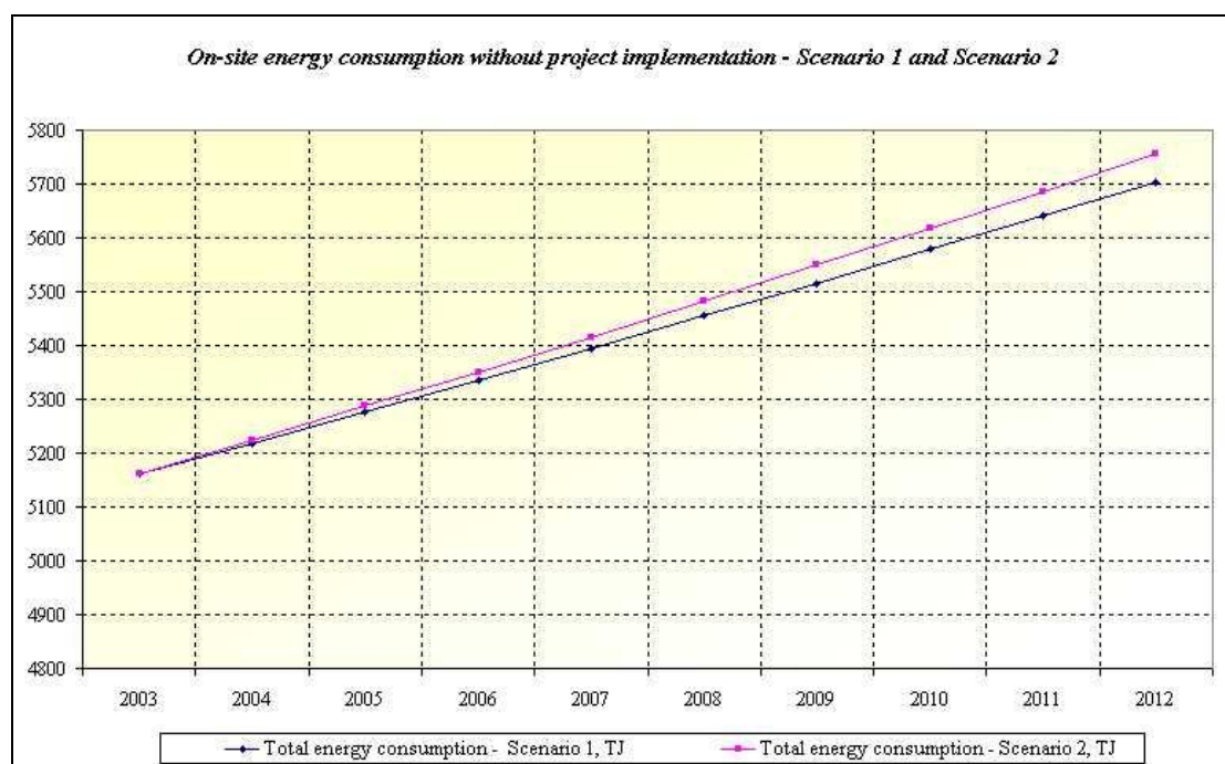
Chart 1: On-site energy consumption without project implementation - Scenario 1 and Scenario 2
